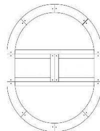
Petite Ox Bow Extended Dining Table w/2 leaves Closed L 1450 x W 900 x H 770 Open (1 inset) L 1800 x W 900 x H 770 Fully open (2 insets) L 2150 x W 900 x H 770
