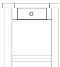
Lamp Table H 550 W 500 D 380
