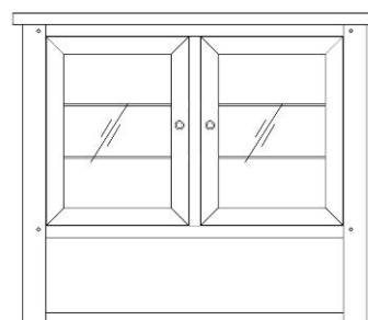
Small Dresser Top H 1076 W 1260 D 380
