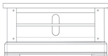
Small TV unit H 450 W 900 D 450
