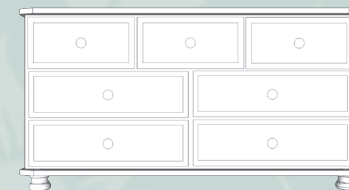
7 DRAWER MULTI-CHEST WTRD131 WPRM131 h:660 w:1180 d:440
